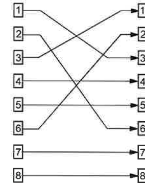
10/100BASE-T (TIA568B)
