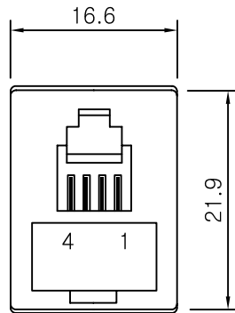
4P4C JACK(L) SIDE VIEW
