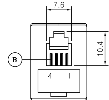
4P4C JACK(R) SIDE VIEW
