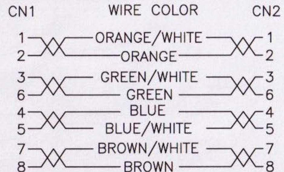
PIN OUT
